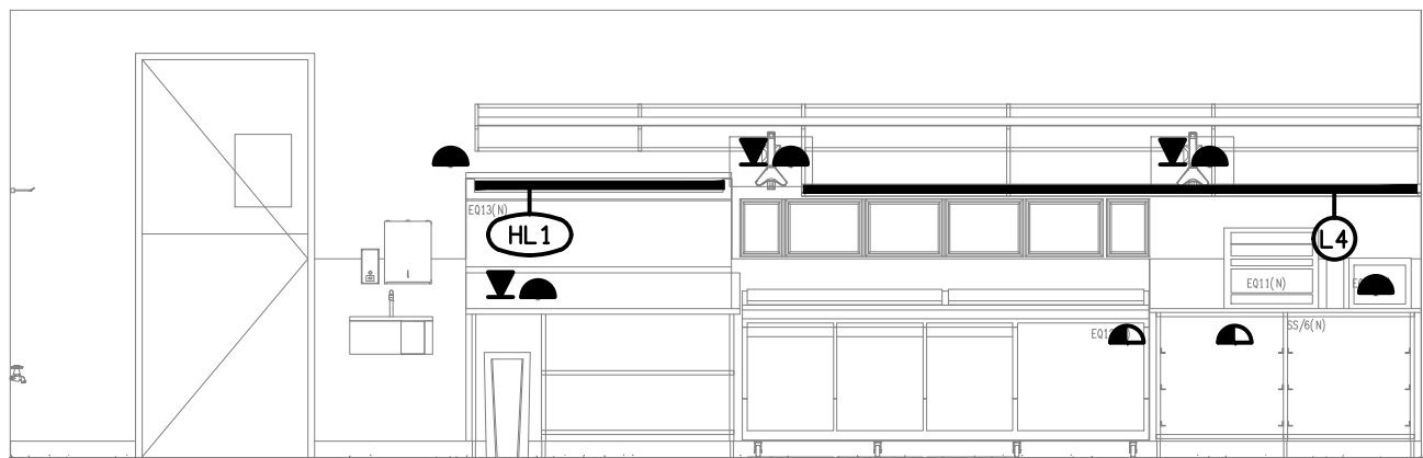
DETAIL 03 BOH MAKELINE ELEVATION SCALE 1: 50
