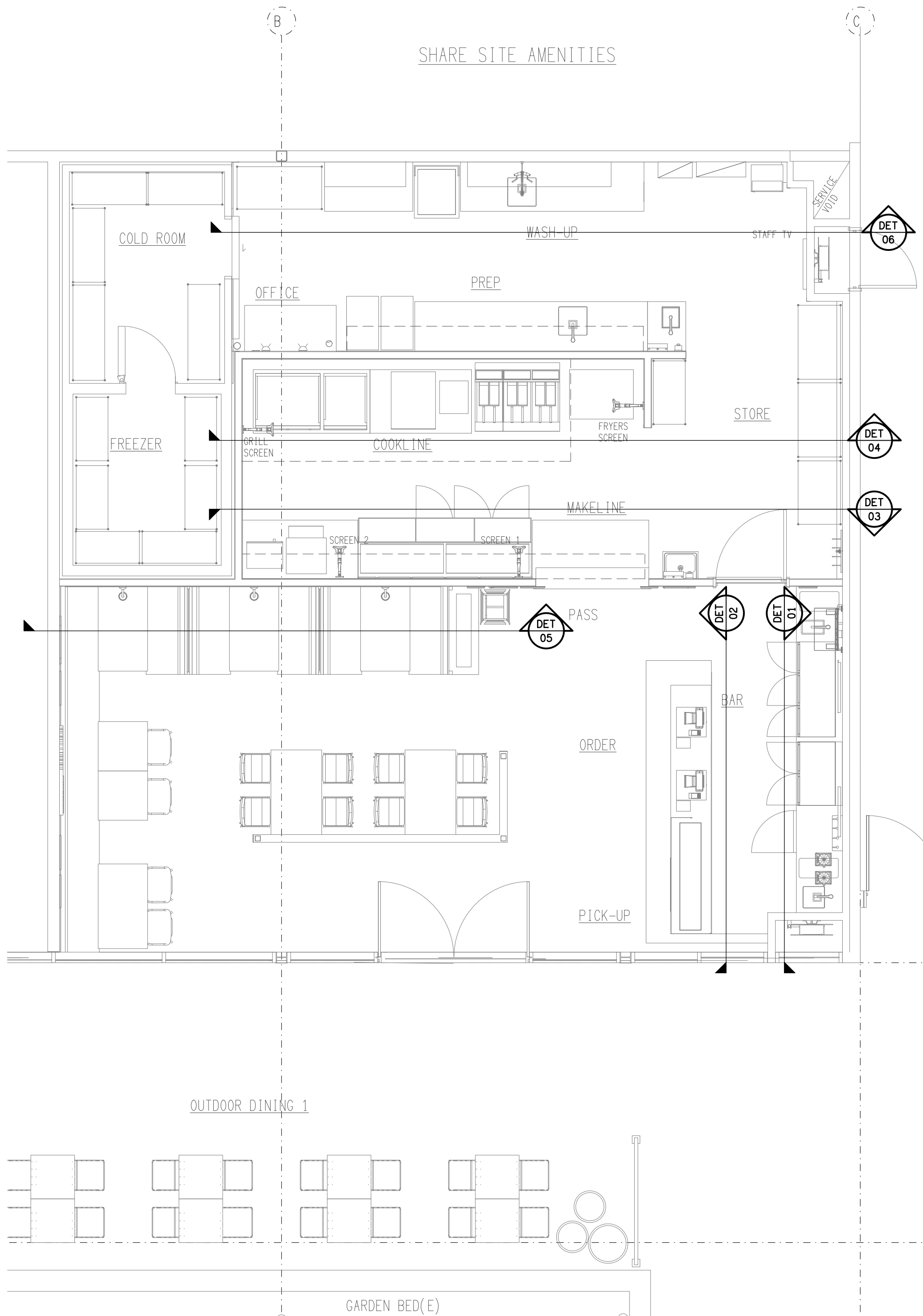
REFERENCE PLAN BURGER URGE TENANCY SCALE 1: 50
